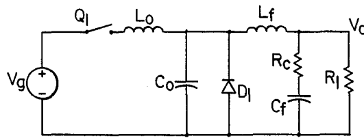
FIG. 1 PRIOR ART
